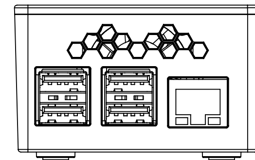
RIGHT VIEW
