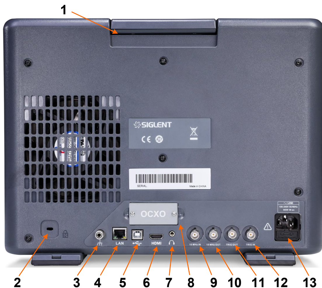
Figure 1-4 Rear Panel
