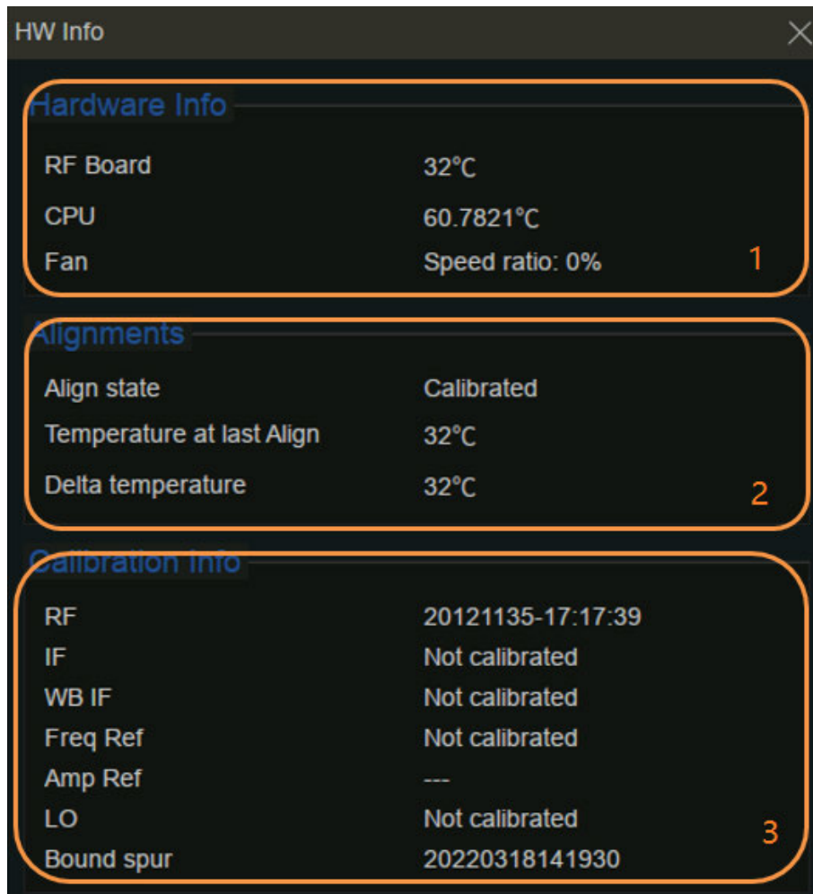
Figure 8-2 Hardware
