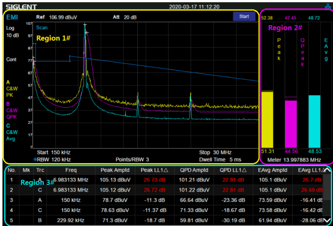
Figure 6-6-1 EMI Measurement User Interface
