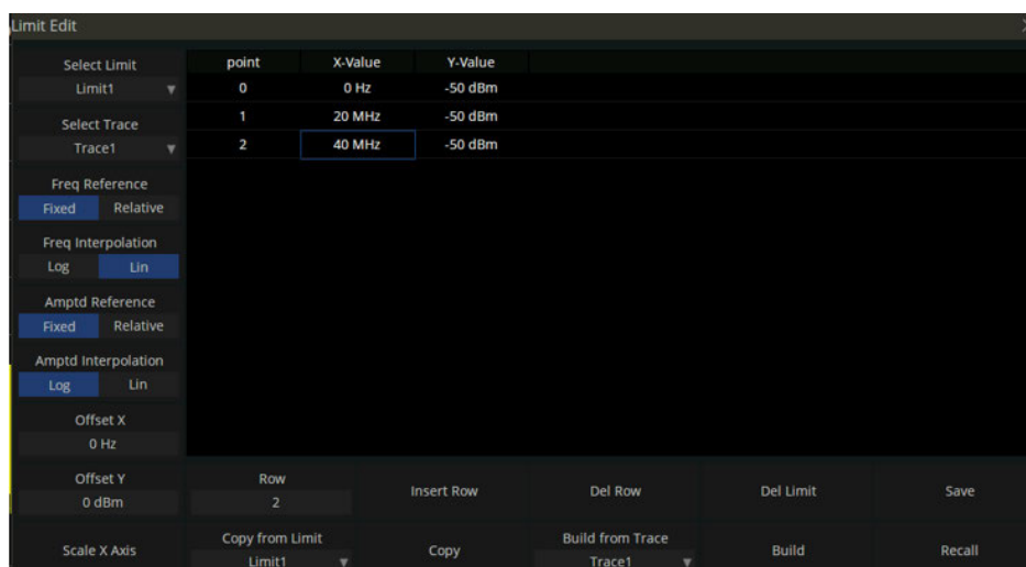
Figure 6-4 limit edit
