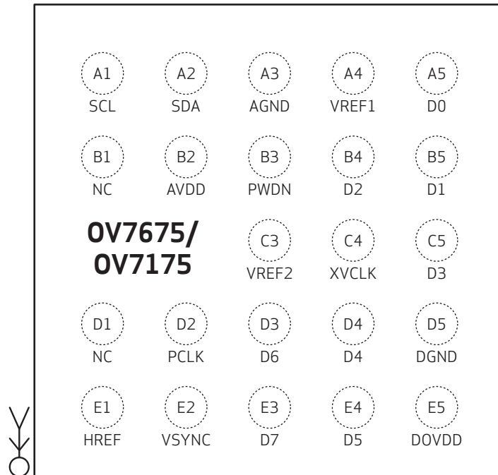
figure 1-1 pin diagram
