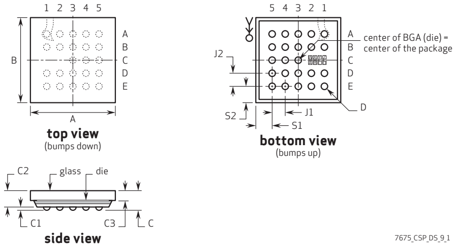
figure 9-1 package specifications
