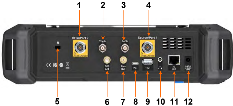
Rear Panel
